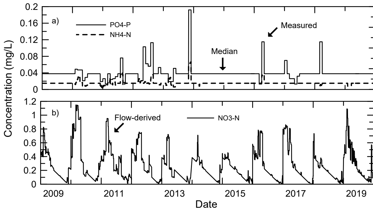
Figure 19. Modeled input nutrient concentrations in Rathbun Creek: a) PO 4 -P and NH 4 -N illustrating use of measured values when available and median values when not, and b) NO 3 -N concentrations derived from regression with total flow rate.
